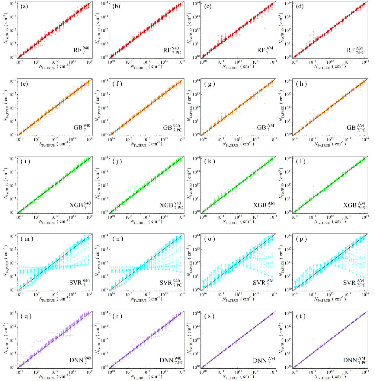
Fig.S5.11. Scatter plots compare reference iron concentrations with ML-predicted values during the N_{\text{Fe}} -altered test in the case of 7D features. The ML algorithms include RF (a-d), GB (e-h), XGB (i-l), SVR (m-p), and DNN (q-t). The data come from simulation under monochromatic (a, b, e, f, i, j, m, n, q, r) and AM1.5 illumination (c, d, g, h, k, l, o, p, s, t). Panels b, d, f, h, j, l, n, p, r, and t include PCA. The black lines are the identified lines serving as the references.
